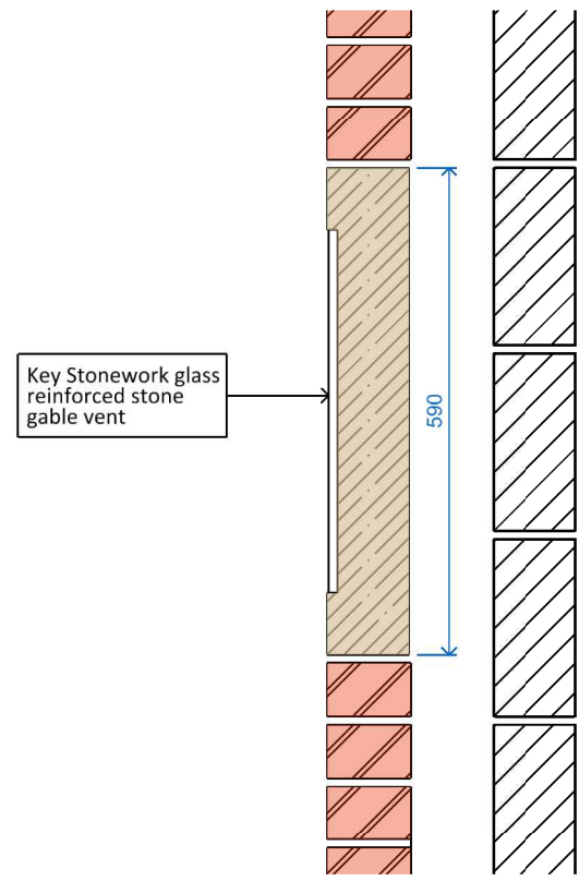
W07 Gable Vent Section (Scale 1:10 @ A1)
