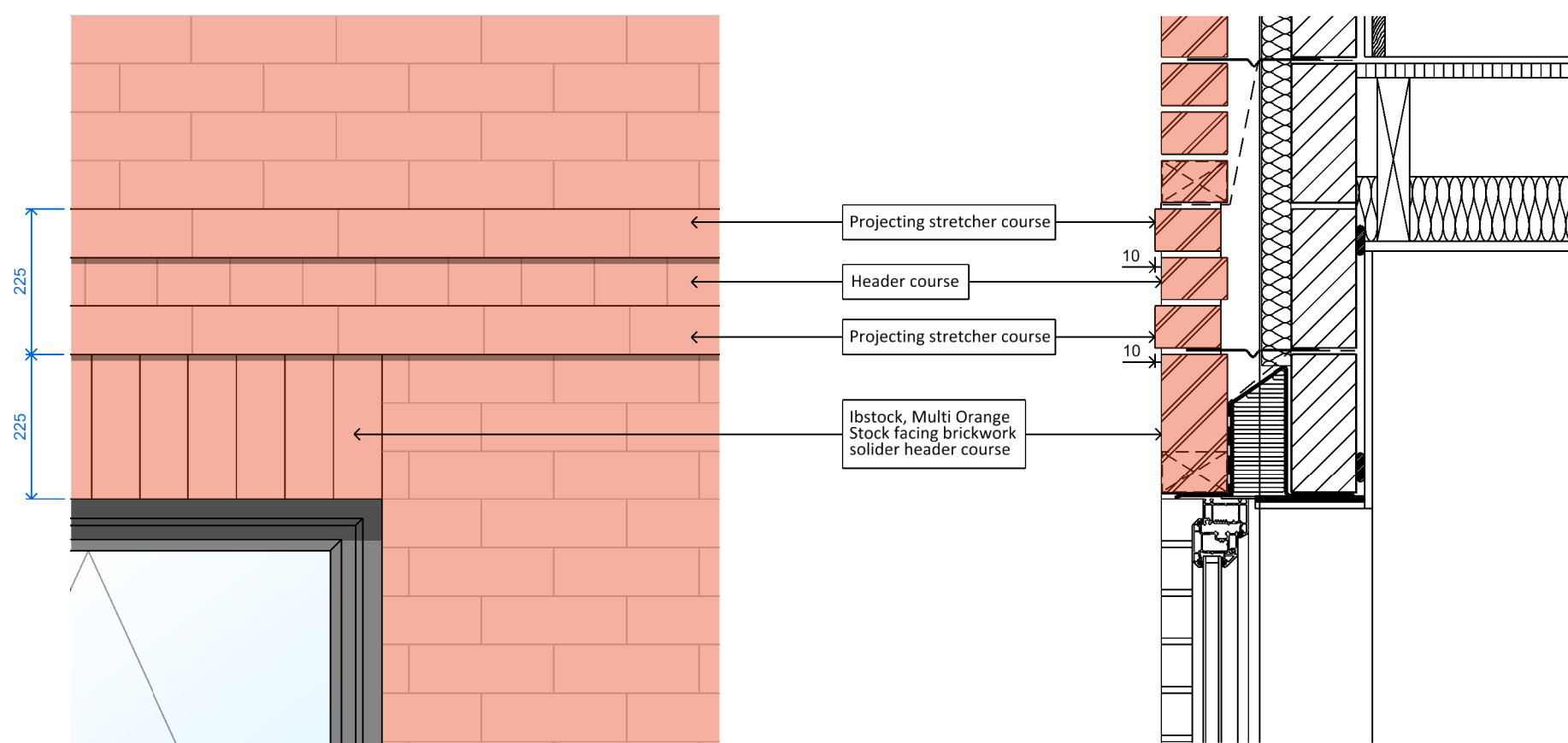
E02 Projecting Brick Band Elevation (Scale 1:10 @ A1)
