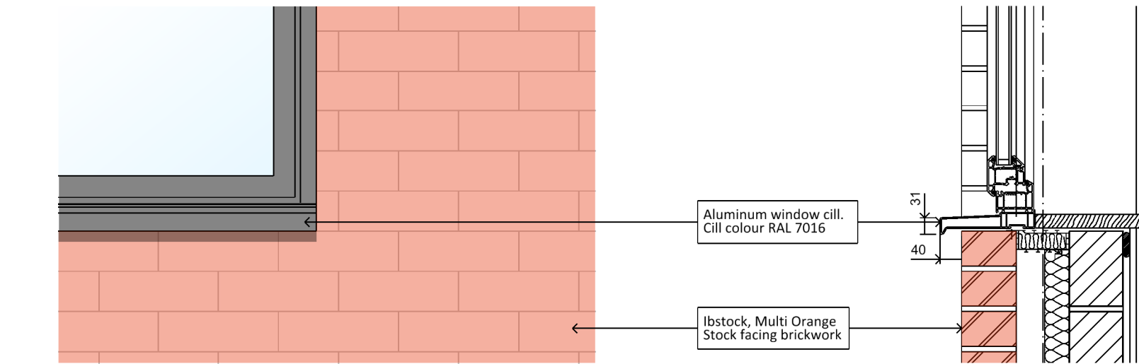
E03 Window Cill Elevation (Scale 1:10 @ A1)
