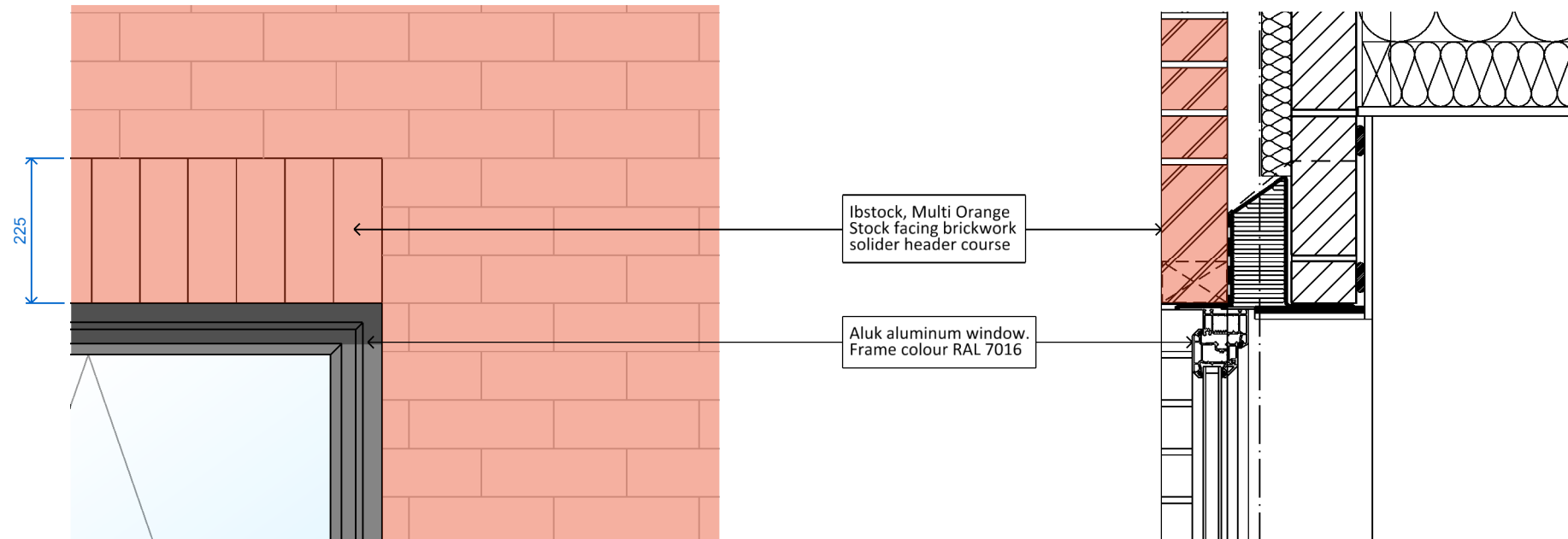
E04 Window Head Elevation (Scale 1:10 @ A1)
