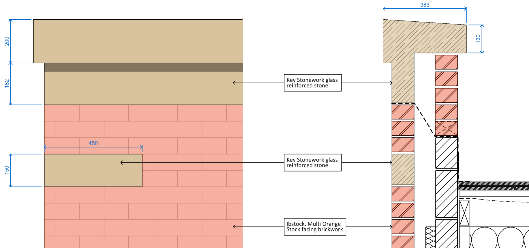
E05 Parapet Coping Elevation (Scale 1:10 @ A1)
