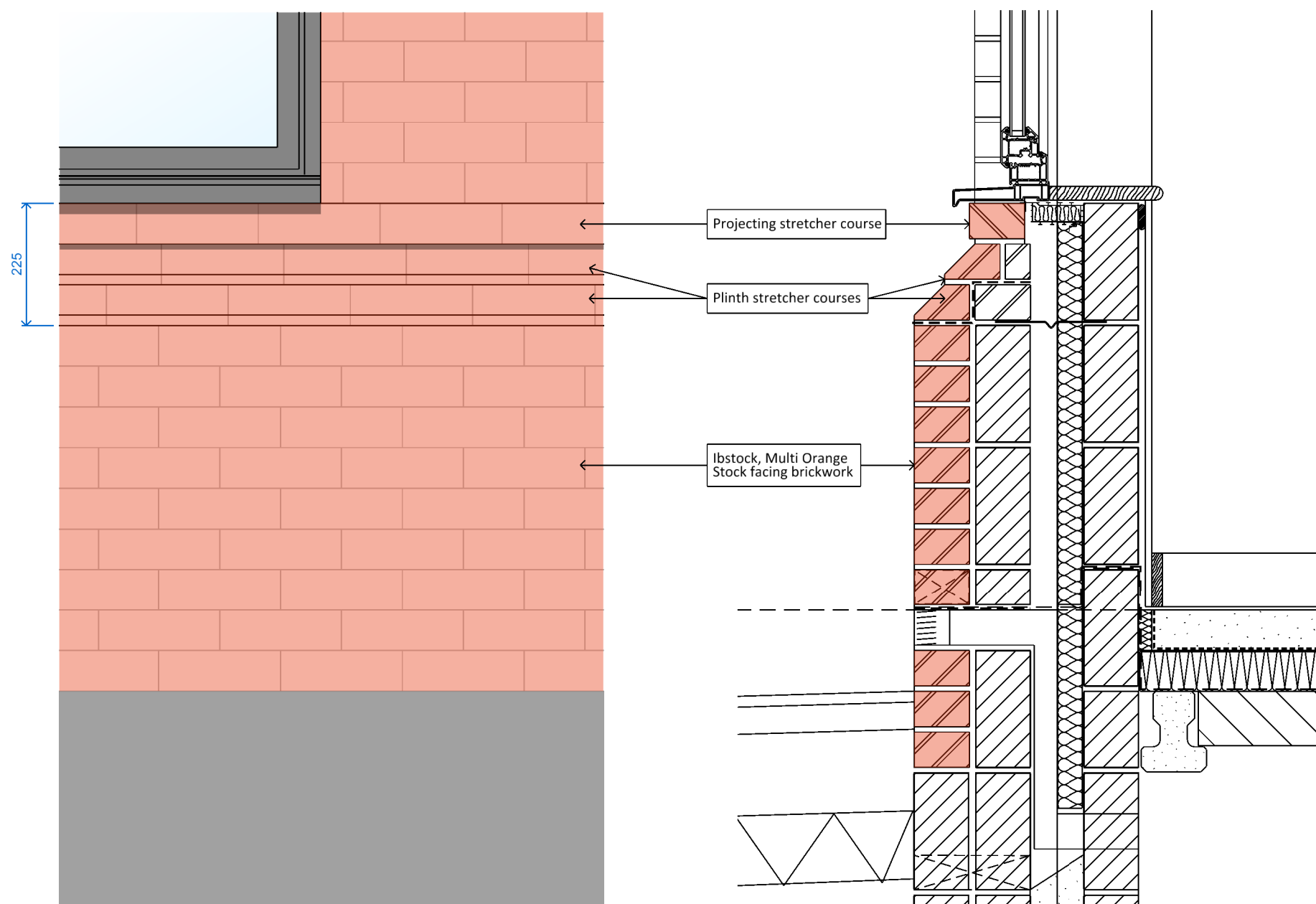
E01 Ground Floor Plinth Elevation (Scale 1:10 @ A1)
